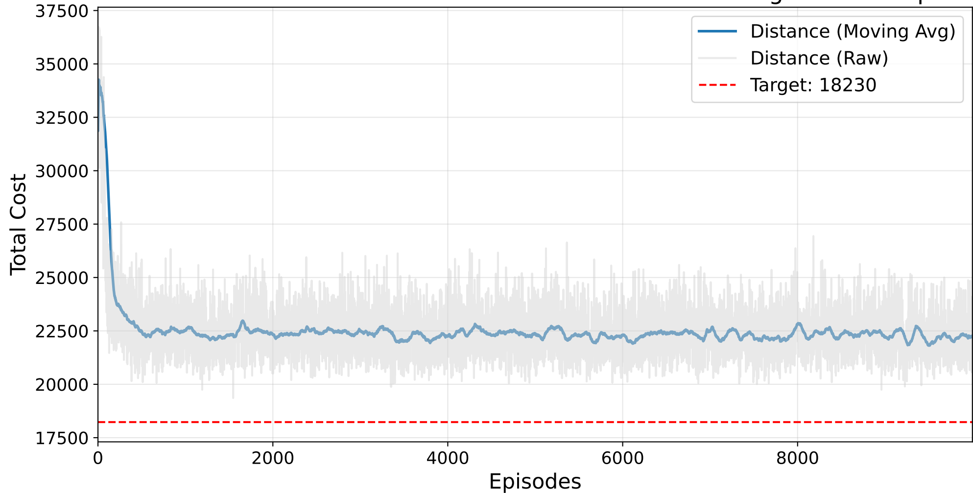
Final GAUSSIAN PROCESS Masked AutoRL-SOP Training - ESC78.sop
